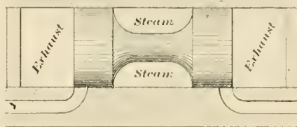
FIG. 3. PISTON VALVE—INSIDE ADMISSION.
